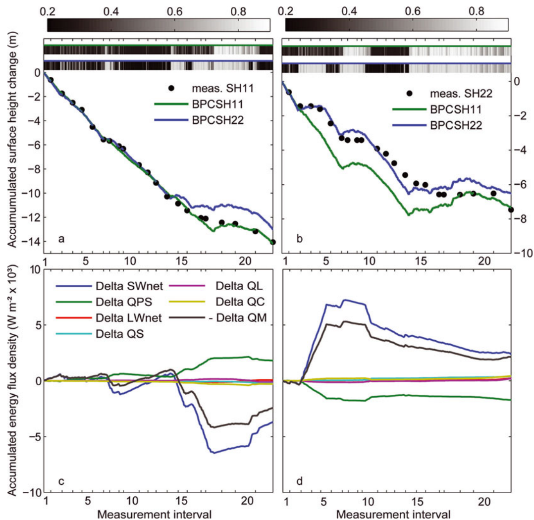
Fig. 7. (a, b) Modeled cumulative relative surface height change from 29 August 2006 to 27 August 2008 with best parameter combinations (BPCs) for each location at SH11 (a) and SH22 (b). Measured values are shown as black dots. Bars at the upper borders of the plots show calculated surface albedo for both runs at hourly time-steps (upper bar is for SH11 run, lower bar for SH22 run). (c, d) Cumulative differences in daily means of energy-balance terms ( SW_{net} and LW_{net} are the net shortwave and net longwave radiation fluxes; the other abbreviations are explained in Section 2.2) for SH11 (c) and SH22 (d). In (c) the values calculated with BPCSH11 are subtracted from BPCSH22, and vice versa in (d). \Delta SW_{in} and \Delta LW_{in} are zero for all runs. For easier readability, \Delta Q_M is multiplied by -1 (since Q_M in the energy balance is negative by sign convention).
